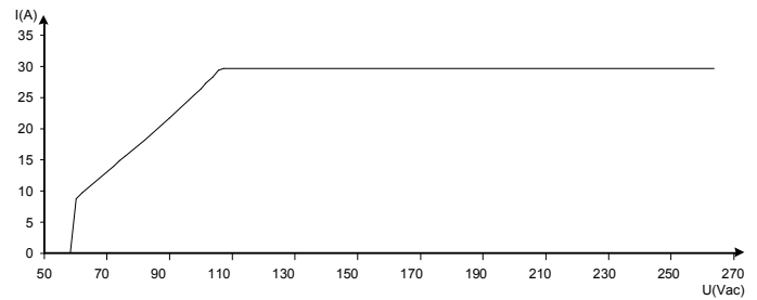
Output current / input voltage de-rating characteristic nominal output
