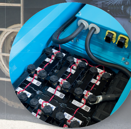
Complete BRIX Batteripack From 24V/80Ah up to 400V and 1000+ Ah
